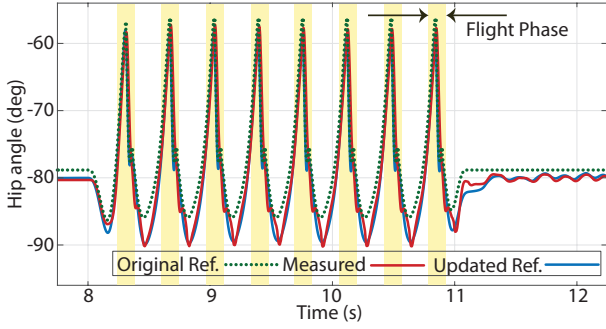
Fig. 10 Hip angle trajectories, experiment #2. The admittance controller updates the reference trajectory in a way so as to contend with contact force errors. The updated reference is q_{ref} := q_{ref} - q_c .
