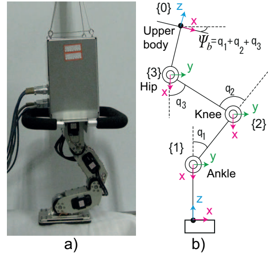
Fig. 1 The actual robot and its joint configurations.
