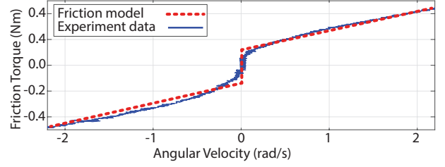
Fig. 6 Experimental friction data vs. identified friction model.
