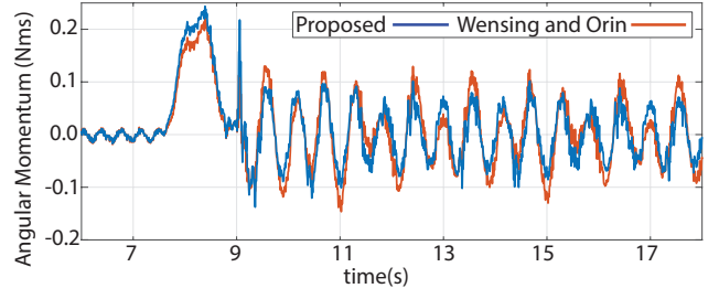
Fig. 4 Angular momentum is computed for a simultaneous squatting-and-swaying motion using EZR and centroidal angular momentum computation algorithm [56].
